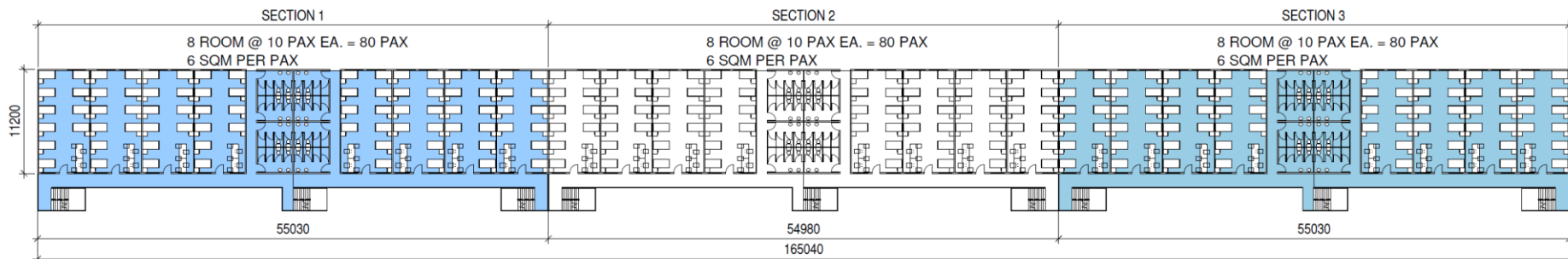
TYPICAL LAYOUT F (6 SQM PER PAX)- 2ND AND 3RD FLOOR N.T.S
